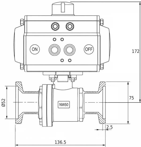
ASSEMBLY DRAWING · UNIT : MM · NW50 ISO-KF CLAMP FLANGE BOTH ENDS · RACK-AND-PINION PNEUMATIC ACTUATOR
