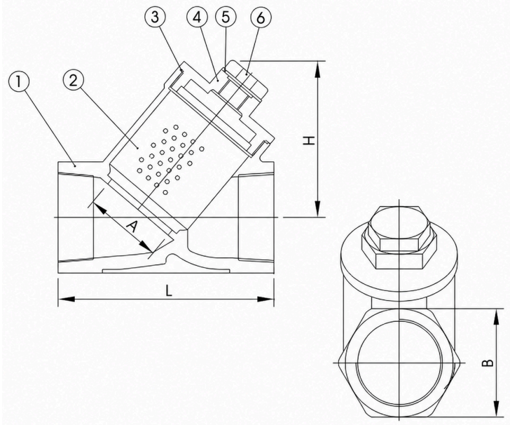
ASSEMBLY DRAWING · UNIT : MM
