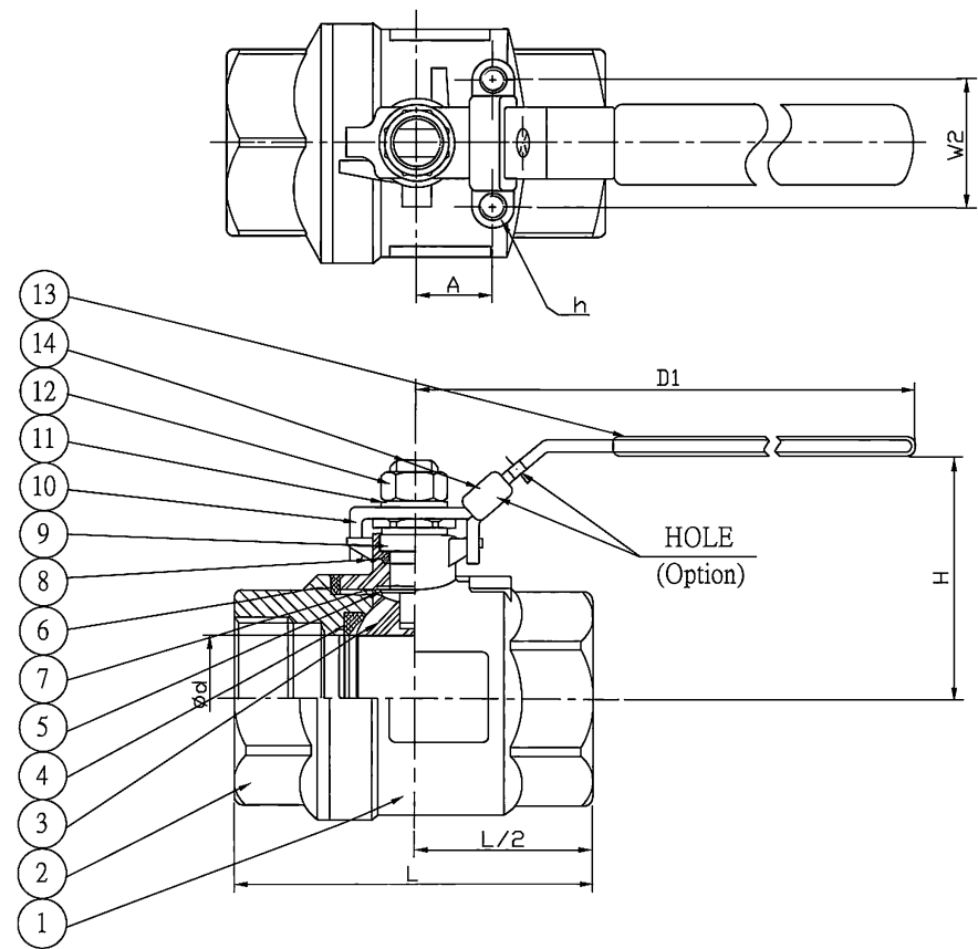
ASSEMBLY DRAWING · UNIT: MM · NO.1-14 → MATERIAL LIST
