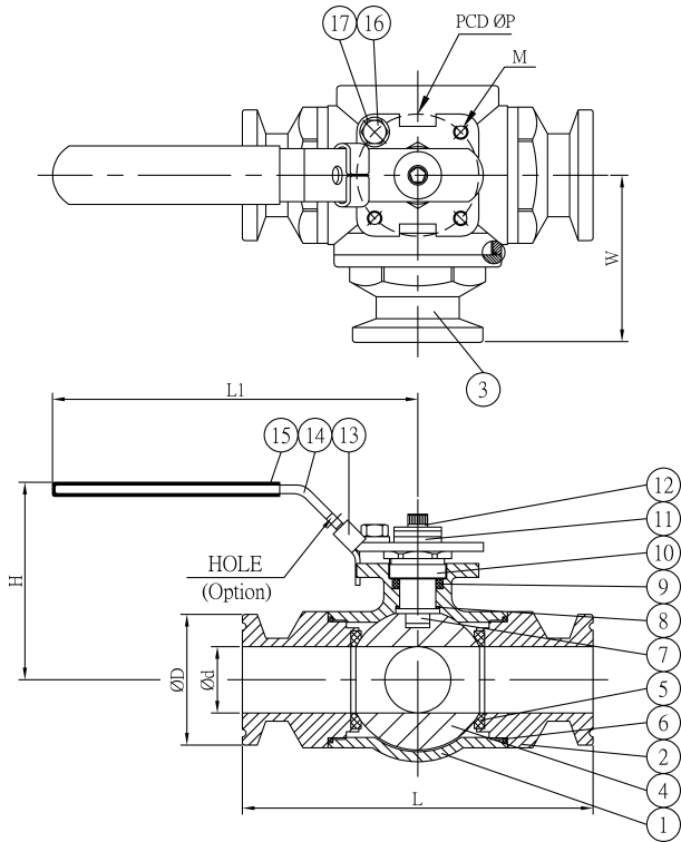
ASSEMBLY DRAWING · UNIT: MM · NO.1-17 → MATERIAL LIST
