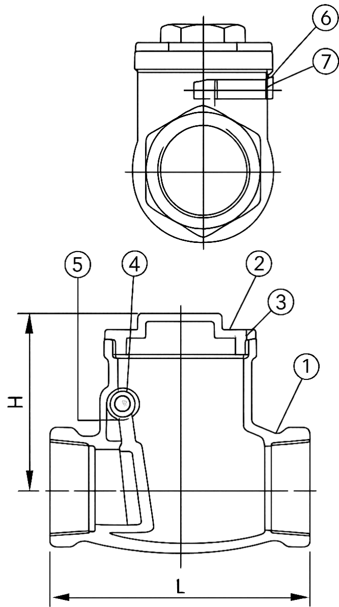
ASSEMBLY DRAWING · UNIT : MM
