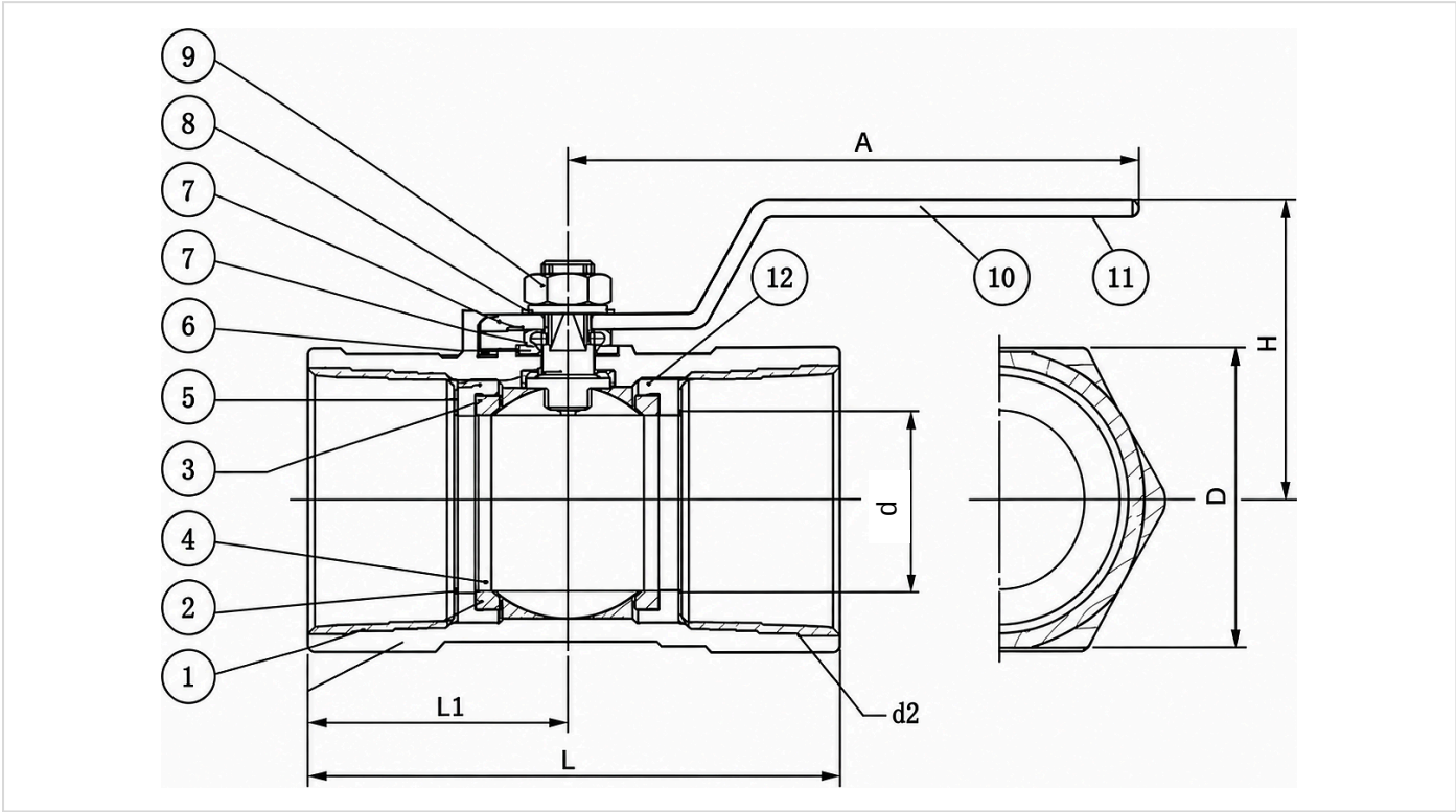
ASSEMBLY DRAWING · UNIT: MM · NO. 1-12 → MATERIAL LIST
