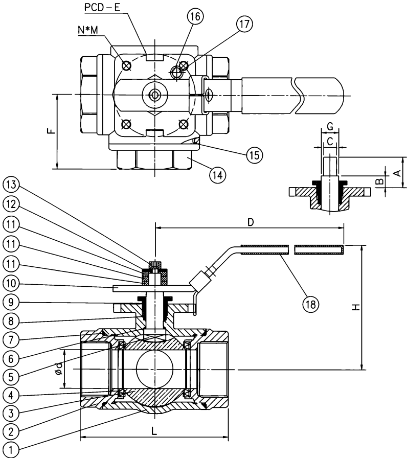
ASSEMBLY DRAWING · UNIT: MM · NO.1-18 → MATERIAL LIST
