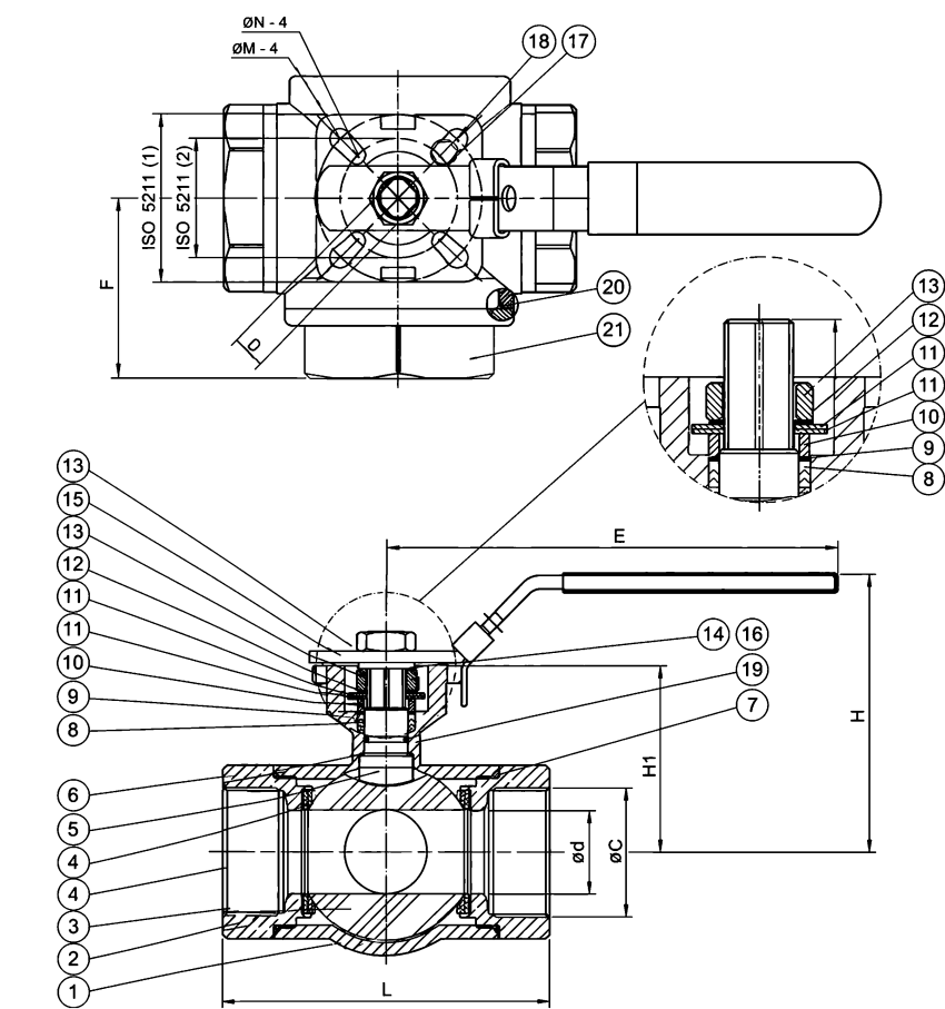
ASSEMBLY DRAWING · UNIT: MM · NO.1-21 → MATERIAL LIST
