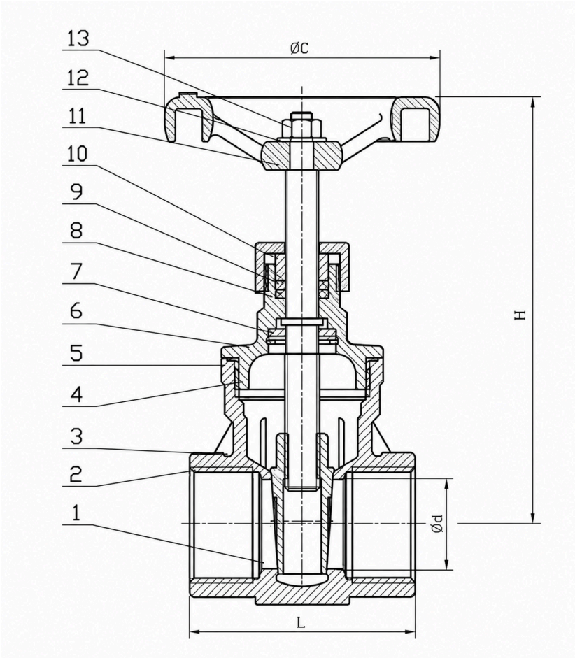
ASSEMBLY DRAWING · UNIT: MM · NO.1-13 → MATERIAL LIST
