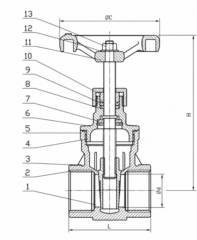
ASSEMBLY DRAWING · UNIT: MM · NO.1-13 → MATERIAL LIST
