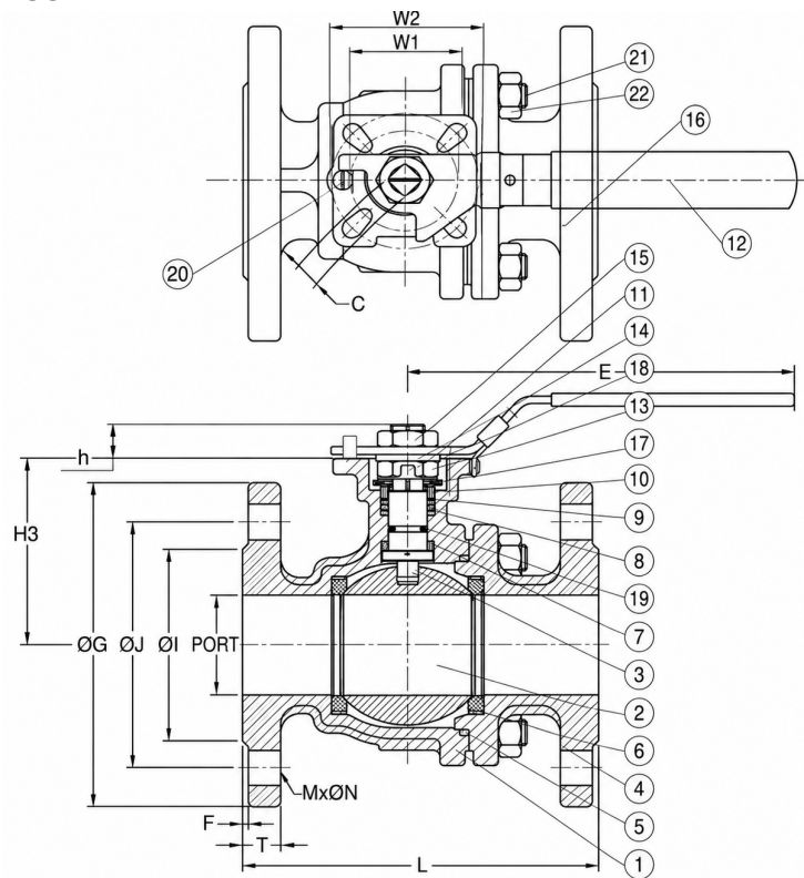
ASSEMBLY DRAWING · UNIT: MM · NO.1-22 → MATERIAL LIST
