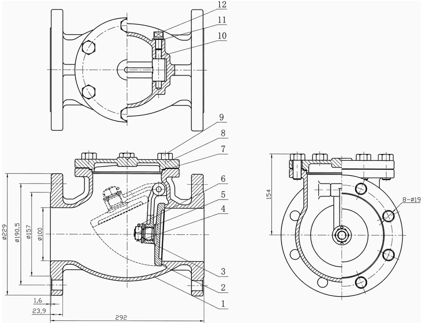
ASSEMBLY DRAWING · UNIT: MM · NO.1-12 → MATERIAL LIST
