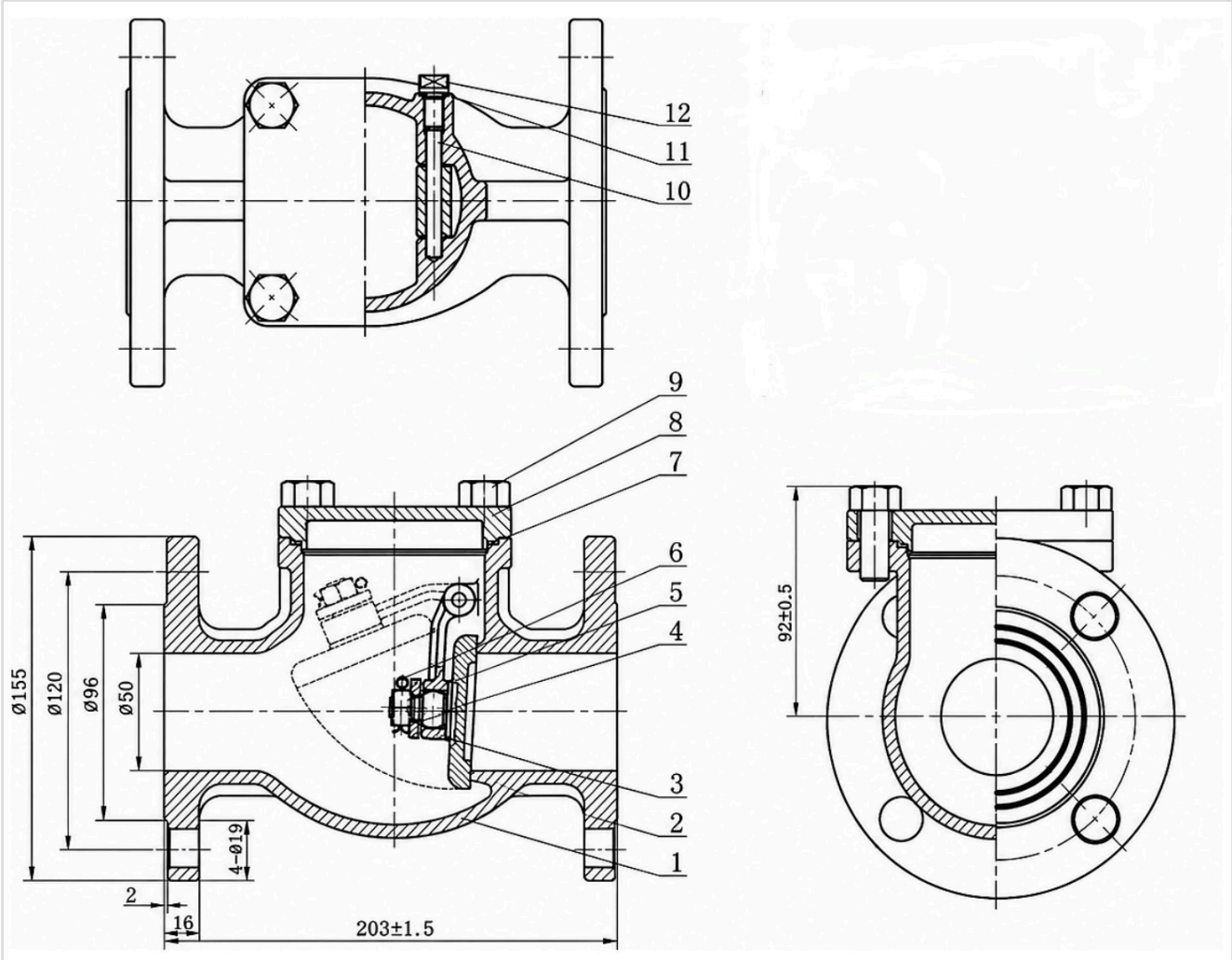
ASSEMBLY DRAWING · UNIT: MM · NO.1-12 → MATERIAL LIST
