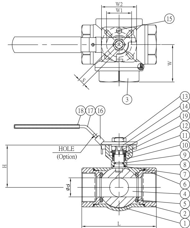
ASSEMBLY DRAWING · UNIT: MM · NO.1-19 → MATERIAL LIST
