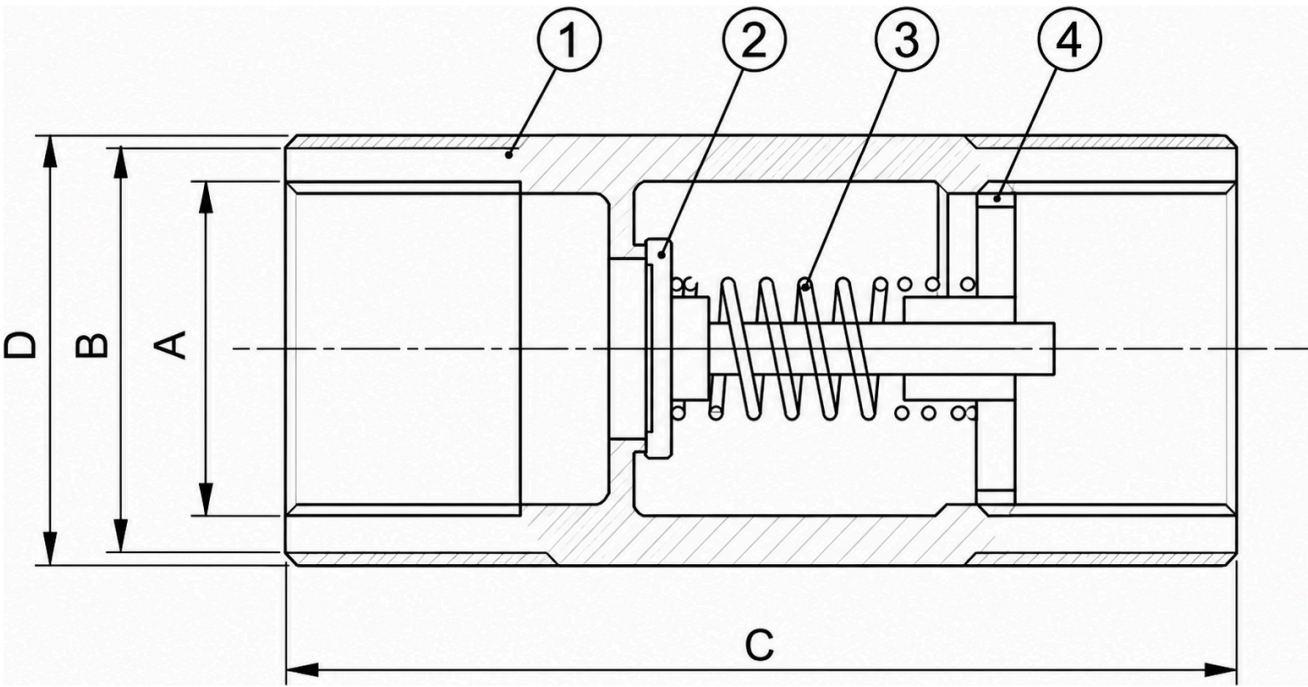
ASSEMBLY DRAWING · UNIT : MM · NO.1-4 → MATERIAL LIST
